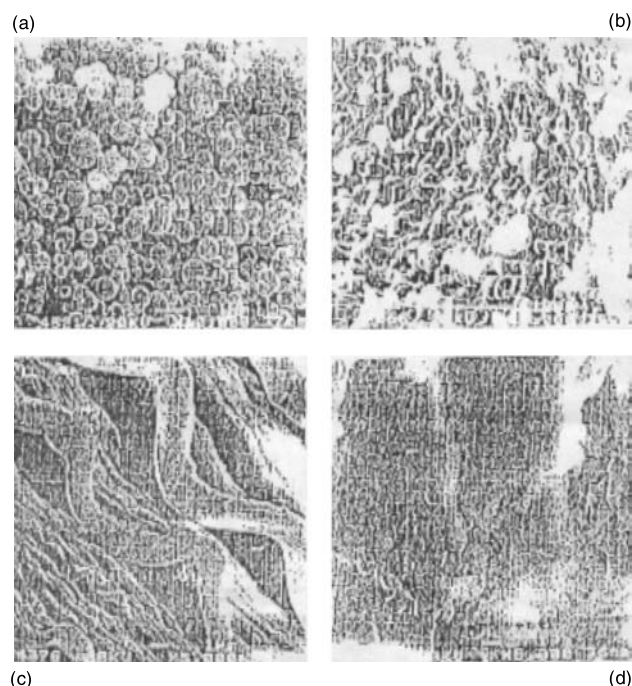
Fig. 3. Scanning electron micrographs of the trunk PAMBN (a), PAMBN-AO (b), polymer complex with \text{Zn}^{\text{II}} (c), and polymer complex with \text{Cu}^{\text{II}} (d) at room temperature
