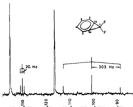
Fig. 1. ^{13}\text{C} -FT-NMR. spectrum of 1,1-difluorobenzocyclopropene (4) in \text{CDCl}_3 at 25.2 MHz ( ^1\text{H} -noise-decoupled)
