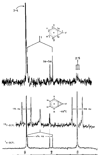
Fig. 2. ^{13}\text{C} -FT-NMR. spectra of 1-fluorobenzocyclopropenium cations at 25.2 MHz in \text{FSO}_3\text{H} at -60^\circ Bottom: ^{13}\text{C} - \{^1\text{H}\} -FT-NMR. spectrum of 6 Center: ^{13}\text{C} - \{^{19}\text{F}\} -FT-NMR. spectrum of 6 Top: ^{13}\text{C} - \{^1\text{H}\} -FT-NMR. spectrum of 6a
