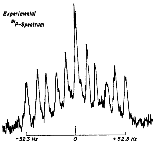
Figure 3. 40.5-MHz ^{31}\text{P} nmr spectrum of neat 1-methylphosphole.
