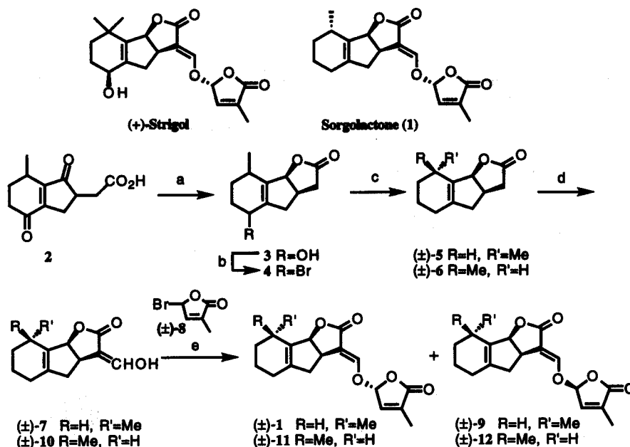
Figure 1. Synthesis of (±)-1
