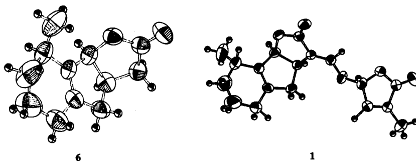
Figure 2. Perspective views of ( \pm )-6 and ( \pm )-1
