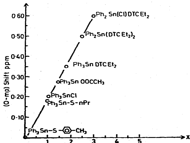
Fig. 2. The effect of different ligands on the ( o-mp ) shift value for phenyl tin complexes.
