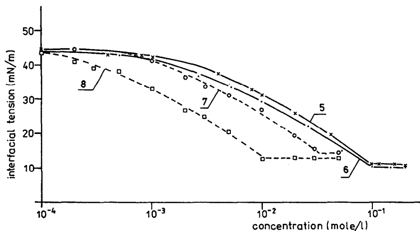
Fig.2. Interfacial tensions (at 25°C) in a water/n-heptane system containing fluoroalkanoates: \text{CF}_3\text{CF}_2\text{CF}_2\text{C}(\text{CF}_3)_2\text{CH}_2\text{COONa} ( 5 ), \text{CF}_3\text{CF}_2\text{CF}_2\text{C}(\text{CF}_3)_2\text{CH}_2\text{CH}_2\text{COONa} ( 6 ), \text{CF}_3(\text{CF}_2)_6\text{COONa} ( 7 ), \text{CF}_3(\text{CF}_2)_7\text{COONa} ( 8 ).
