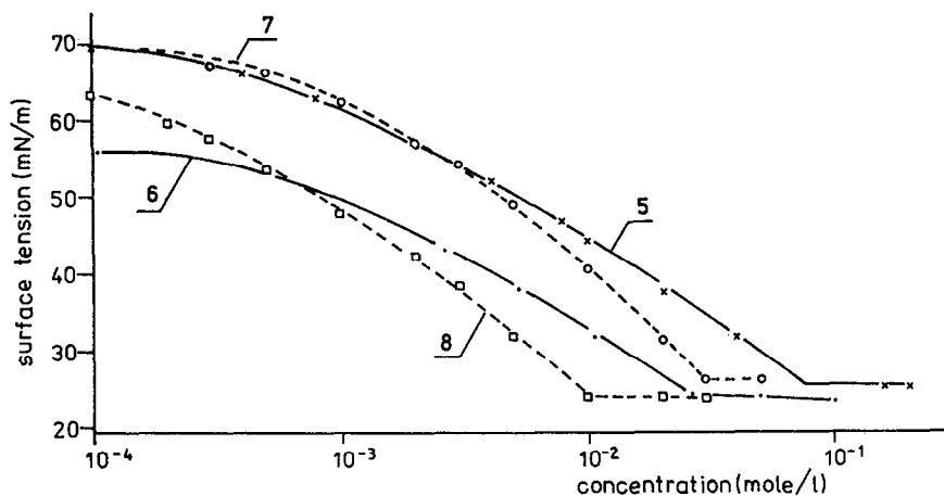
Fig.1. Surface tensions (at 25°C) of aqueous solutions of fluoroalkanoates: \text{CF}_3\text{CF}_2\text{CF}_2\text{C}(\text{CF}_3)_2\text{CH}_2\text{COONa} ( 5 ), \text{CF}_3\text{CF}_2\text{CF}_2\text{C}(\text{CF}_3)_2\text{CH}_2\text{CH}_2\text{COONa} ( 6 ), \text{CF}_3(\text{CF}_2)_6\text{COONa} ( 7 ), \text{CF}_3(\text{CF}_2)_7\text{COONa} ( 8 ).
