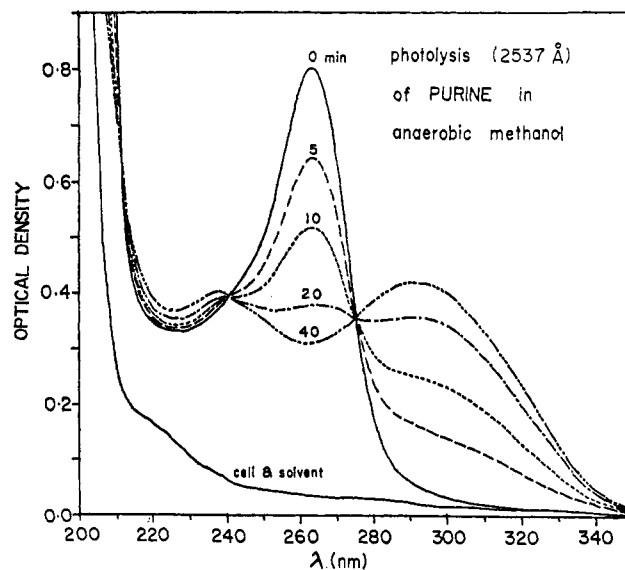
Figure 1. Spectral changes during photolysis (2537 Å) of purine in degassed methanol. Initial purine concentration 7.0 \times 10^{-5} M ; I_0 = 6 \times 10^{-8} einstein/(cm 2 min); cell path = 14.7 mm; time in minutes.
