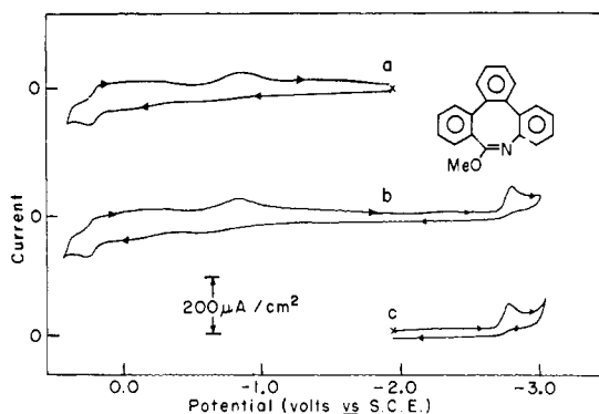
Figure 2. Cyclic voltammetry of 3.35 \times 10^{-5} M TBMA (3) at a stationary Pt-bead electrode in dry THF solvent. Background 0.2 M TBAHFP, scan rate, 400 mV/sec; \times indicates initial potential; a, positive going single sweep; b, steady state (free run); c, negative going single sweep.
