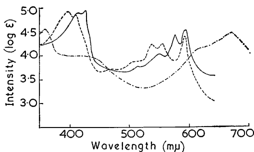
FIG. 2. Visible absorption spectra of 8,12-diethyl-2,3,7,13,17,18-hexamethylcorrole in NN -dimethylformamide (-----), NN -dimethylformamide containing one drop of 1% aqueous sodium hydroxide (—), and in concentrated sulphuric acid (— · — · —)
