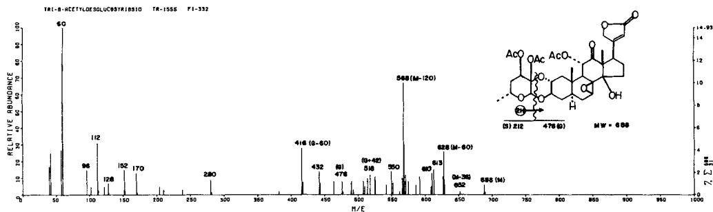
Fig. 10. FI-mass spectrum of tri-O-acetyl-desgluco-syrioside (13=TR-1555), m.p. 302–303°, C_{35}H_{44}O_{14} (688) with hypothetical genin C_{25}H_{32}O_9 (476), probe temp. 270°. Assignments: 688 ( M ); 652 (688–18–18); 628 (688–60); 613 (628–15); 610 (628–18); 592 (610–18); 586 (628–42); 568 (628–60); 550 (568–18); 526 (568–42); 518 ( G + 42); 508 (568–60); 490 (508–18); 476 ( G ); 464; 432 (476–44); 416 ( G – 60); 280 (?); 170 (43); 152 (170–18); 128 (18).
