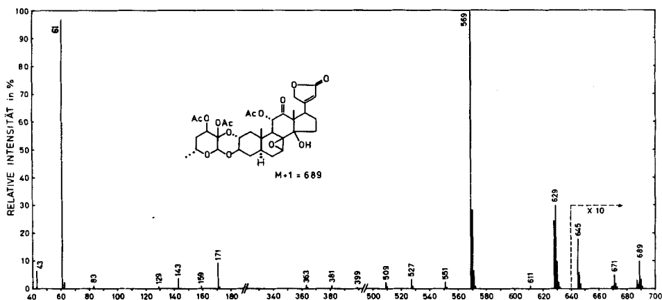
Fig. 11. H_2 -CI-mass spectrum 15 of tri-O-acetyl-desgluco-syrioside (13=TR-1555B), m.p. 302–303°, C_{35}H_{34}O_{14} (688), source temp. 230°, probe temp. 190°. Assignments: 689 ( M + H^+ ); 671 (689–18); 645 (689–44 or M –1–42); 629 (689–60); 611 (629–18 and 671–60); 587 (629–42); 569 (629–60); 551 (569–18 and 611–60); 527 (569–42 and 587–60); 509 (527–18, 551–42 and 569–60); 459 ( G –18 + H , R.A. < 1%); 399 (569–170 or 527–128, corr. to G –60–18 + H^+ ); 381 (399–18 or 551–170 or 509–128); 363 (381–18); 171 (45); 129 (171–42); 143 (171–28); 83 (143–60). Peaks for G + H^+ (477) and mono- O -acetyl- G + H^+ (519) were absent. The ions at m/e 143 and 83 are probably derived from 45 and may best be represented by 51 and 52. Observation of the key ion peaks at 689 ( M + H ); 629 ( M + 1–60); 569 ( M + 1–60–60) and 509 ( M + 1–60–60–60) provides strong evidence for the presence of 3 acetoxy groups in 13.
