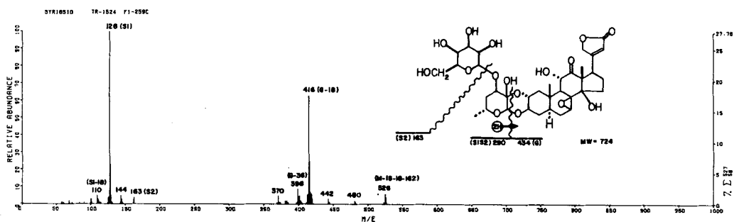
Fig. 6. FI-mass spectrum 14 of syrioside (10=TR-1524), m.p. 230–231°, C_{35}H_{48}O_{16} (724), probe temp. 235°. Assignments: 526 (M–18–180 ( C_6H_{12}O_6 =glucose)); 416 (G–18); 398 (416–18); 370 (398–28); 163 ( C_6H_{11}O_5 =glycosyl cation); 128 (18).
