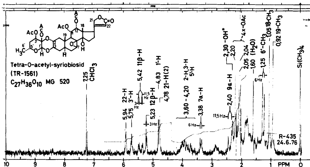
Fig. 14. 100-MHz-NMR. spectrum of tetra-O-acetyl-syriobioside (8=TR-1561), m.p. 338-340° in CDCl_3 17 . Contained one mol water of crystallisation. Assignments tentative.
