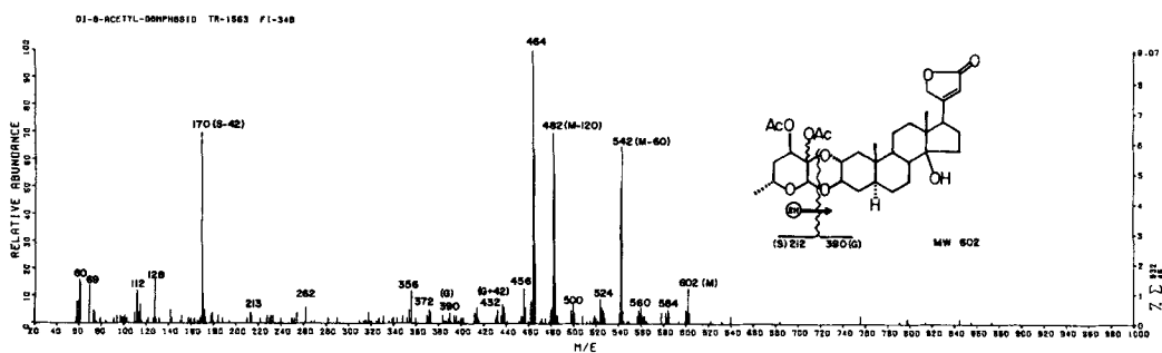
Fig. 7. FI-mass spectrum 14 of di-O-acetyl gomphoside (21=TR-1563 purified by chromatography on SiO_2 ), m.p. 285–287°, C_{33}H_{46}O_{10} (602), probe temp. 220°. Assignments: 602 (M); 584 (M–18); 560 (M–42); 542 (M–60); 524 (542–18); 500 (542–42); 482 (M–120); 464 (482–18); 456 (500–44); 432 (G+42); 390 (G); 372 (G–18); 356 (?); 170 (43).
