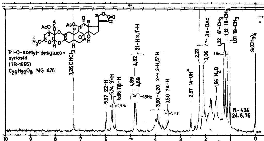
Fig. 16. 100-MHz-NMR. spectrum of tri-O-acetyl-desgluco-syrioside (13 = TR-1555-A), m.p. 300–301° (decomp.) in CDCl_3 17 ), containing some water of crystallisation. Assignments tentative
