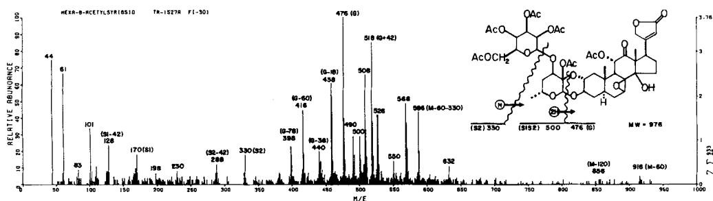
Fig. 12. FI-mass spectrum of hexa-O-acetyl-syrioside (11=TR-1527A), m.p. 192–193°, C 47 H 60 O 22 (976), probe temp. 265°. Assignments: M + not visible; 916 ( M – 60); 856 (916 – 60); 632 (?); 586 (916 – 330); 568 (586 – 18); 550 (568 – 18); 526 (568 – 42); 518 ( G + 42); 508 (568 – 60); 500 (S1S2; 518 – 18); 490 (550 – 60); 476 ( G ); 458 ( G – 18); 440 ( G – 18 – 18); 416 ( G – 60); 398 (416 – 18); 330 (S2); 288 (330 – 42); 170 (43); 128 (170 – 42); 110 (170 – 60; 128 – 18).
