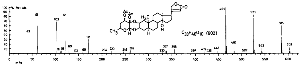
Fig. 8. H_2 -CI-mass spectrum 15 of di-O-acetyl-gomphoside (21), source temp. 220°, probe temp. 180°. Assignments: 603 ( M+H^+ ); 585 (603-18); 543 (603-60 and 585-42); 525 (585-60); 501 (543-42); 483 (543-60); 465 (525-60 and 483-18); 447 (465-18); 429 (447-18); 397 (525-128); 355 (483-128 and 525-170, corresp. to 47 (= G-36)+ H^+ ); 337 (465-128 and 355-18 and 525-170); 171 (43); 129 (171-42); 111 (129-18). The processes summarized in Scheme 1 could be confirmed by metastable peaks in defocussed spectra.
