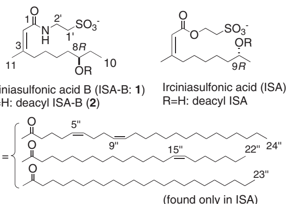
Figure 1. Structures of ISAs.
