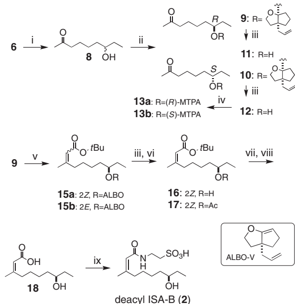
Scheme 2. Reagents and conditions: (i) H_2 , Rh- Al_2O_3 , EtOH, 0 °C, 3 h, 72%; (ii) ALBO-V, PPTS, CH_2Cl_2 , rt, 1.5 h, 9 : 45%, 10 : 50%; (iii) PPTS, MeOH, rt, 11 : 68%, 12 : 85%, 16 : 45%; (iv) (R)- or (S)-MTPACl, pyridine, rt, 3.5 h; (v) (EtO)_2P(O)CH_2COOt-Bu ( 14 ), KOt-Bu, THF, 0 °C–rt, 12 h, 15a : 11%, 15b : 60%; (vi) Ac_2O , pyridine, rt; (vii) TFA, CH_2Cl_2 , rt; (viii) 0.1 M NaOMe, MeOH, rt, 84% (yield of vi–viii); (ix) taurine, DMT-MM, N -methylmorpholine, acetone/ H_2O , rt, 12 h, 46%.
