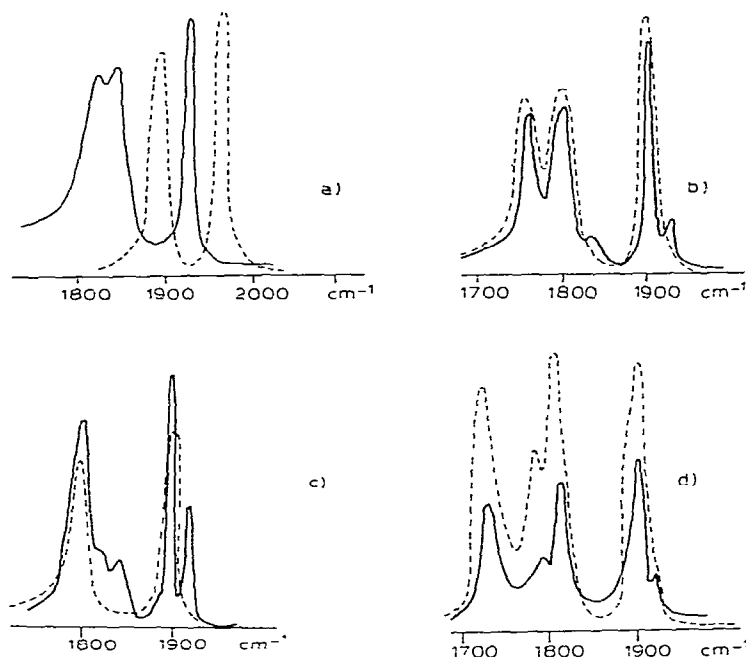
Fig. 1. Absorption IR spectra in the \nu(\text{CO}) region. (a) — \eta^6\text{-C}_{13}\text{H}_9\text{Cr}(\text{CO})_3^-\text{K}^+ in THF at -40^\circ\text{C} ; - - - \eta^6\text{-fluorenechromium tricarboxyl} in THF; (b) — equilibrium mixture of the K salts of I and II at 28^\circ\text{C} in THF; - - - \eta^5\text{-C}_5\text{H}_5(\text{CO})_3\text{Cr}^-\text{K}^+ in THF; (c) — equilibrium mixture of the K salts of I and II in the presence of crown ether IV (THF, 28^\circ\text{C} ); - - - \eta^5\text{-C}_5\text{H}_5(\text{CO})_3\text{Cr}^-\text{K}^+ in the presence of IV; (d) — \eta^5\text{-C}_{13}\text{H}_9(\text{CO})_3\text{Cr}^-\text{Li}^+ in THF; - - - \eta^5\text{-C}_5\text{H}_5(\text{CO})_3\text{Cr}^-\text{Li}^+ in THF.
