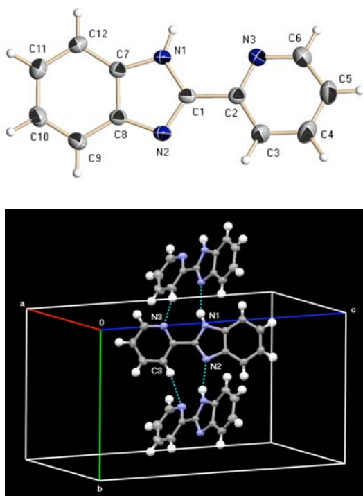
Figure 1. Perspective of the molecular structure of compound 1 and illustration of the most relevant hydrogen-bonding interactions within the crystal lattice.
