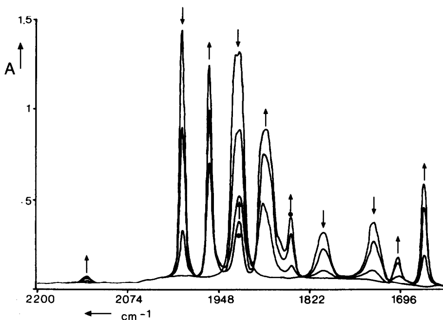
Fig. 5. IR-spectral changes in the CO-stretching region during the photochemical reaction of [\text{Fe}_2(\text{CO})_6(\text{bipy})(\text{P}(\text{n-Bu})_3)] with pyridine at 133 K in 2-Me-THF (● = decomposition product).
