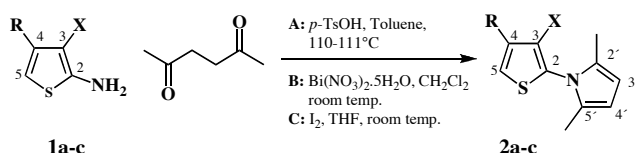
Figure 2. Paal-Knorr reaction of substituted 2-aminothiophenes.
