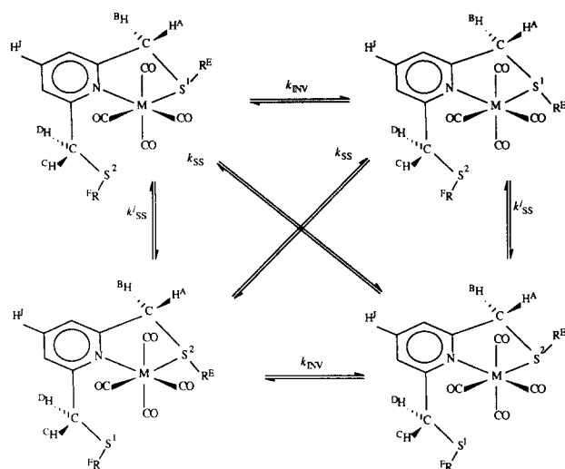
Fig. 2. Four permutational isomers of the complexes [M(CO)_4L] ( L = L^1 or L^2 ) showing their interconversions resulting from inversion of the coordinated S atom, fluxional S^1-S^2 switching of the ligand, and combined S inversion and S^1-S^2 switching.
