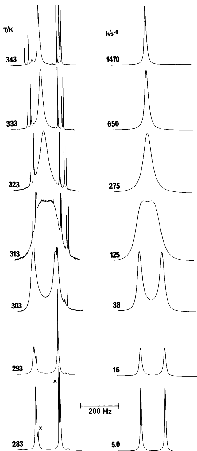
Fig. 3. Variable temperature ^1\text{H} NMR spectra of the ligand methyl signals of [\text{W}(\text{CO})_4\text{L}^1] , with computer-simulated spectra and “best-fit” rate constants, k_{\text{obs}} , shown alongside. Two impurity signals depicted by X.
