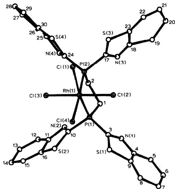
Fig. 2. Structure of [\text{RhCl}_4(\text{BTPE})]^- . Selected bond distances (Å) and angles ( ^\circ ) are: Rh(1)–Cl(1), 2.45(2); Rh(1)–Cl(2), 2.33(2); Rh(1)–Cl(3), 2.36(2); Rh(1)–Cl(4), 2.39(2); Rh(1)–P(1), 2.22(2); Rh(1)–P(2), 2.18(2); Cl(1)–Rh(1)–Cl(2), 91.0(6); Cl(1)–Rh(1)–Cl(3), 92.1(6), Cl(1)–Rh(1)–Cl(4), 96.7(6); Cl(1)–Rh(1)–P(1), 169.9(7); Cl(1)–Rh(1)–P(2), 85.6(7).
