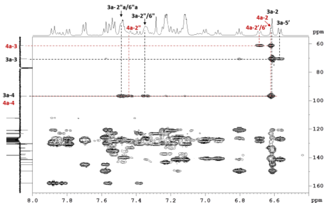
Figure 2: ^1\text{H} - ^{13}\text{C} NMR HMBC experiment of 3a and 4a in \text{CDCl}_3
