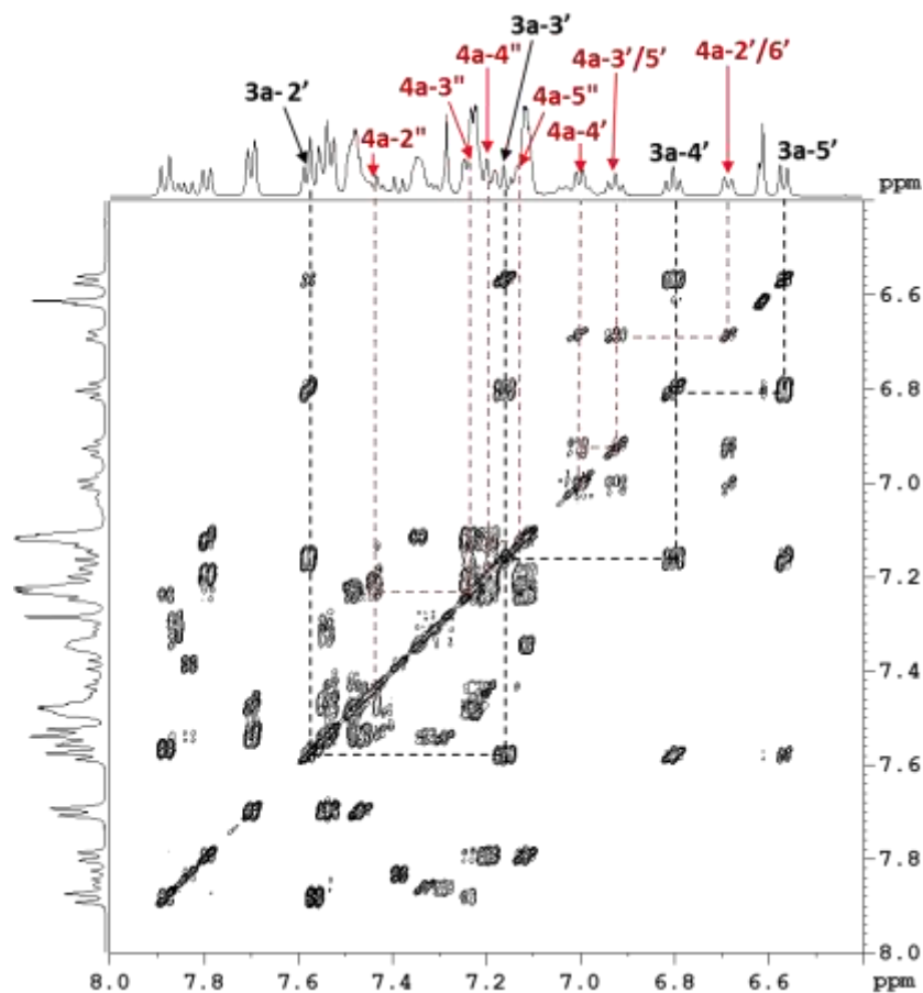
Figure 1: ^1\text{H} - ^1\text{H} NMR COSY experiment of 3a and 4a in \text{CDCl}_3
