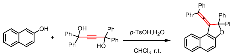
Scheme 1: Synthesis of vinylidene-naphthofuran from 2-naphthol and tetraphenylbut-2-yne-1,4-diol.
