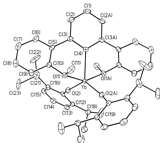
Figure 4. ORTEP diagram of \text{DanipYb}[\text{O}(2,6\text{-diisopropylphenyl})]_2 ( 4 ) showing the atom-labeling scheme. Thermal ellipsoids are at the 30% level. Hydrogen atoms were omitted for clarity.
