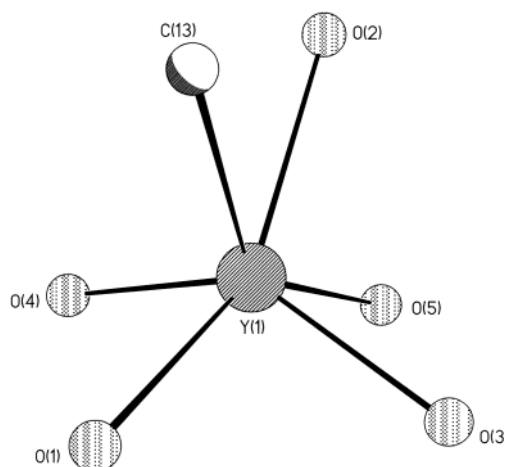
Figure 6. Central core of 5a showing the distorted trigonal-prismatic coordination polyhedron.
