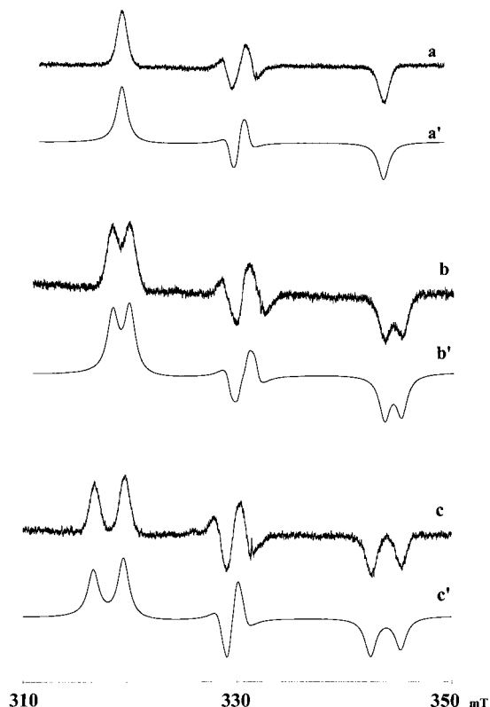
Figure 2. EPR spectra obtained at 110 K with an electrochemically reduced solution of (a) \text{ArP}=\text{C}=\text{C}(\text{C}_6\text{H}_5)_2 , (b) \text{ArP}=\text{}^{13}\text{C}=\text{C}(\text{C}_6\text{H}_5)_2 , (c) \text{ArP}=\text{C}=\text{}^{13}\text{C}(\text{C}_6\text{H}_5)_2 . a', b', and c' are the corresponding simulated spectra (see text).
