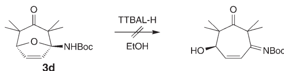
Scheme 6. Attempt to Obtain a Monocyclic Intermediate by Deprotonation of the BocNH Group
