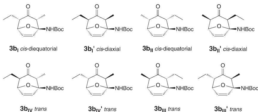
Fig. 2. Possible formation of eight different isomeric cycloadducts, according to the proposed mechanism, from nonsymmetric \alpha,\alpha' -dihalo ketone 1b
