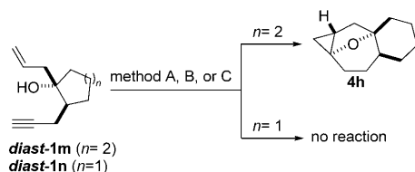
Scheme 5. Cycloisomerization reactions of alkynols diast-1m and diast-1n . Method A: 25 mol % preformed [(thf)W(CO) 5 ], THF, RT; method B: 10 mol % [W(CO) 6 ], 2 mol % Et 3 N, THF, 50 °C, hν ; method C: 10 mol % [W(CO) 6 ], 200 mol % Et 3 N, THF, 50 °C, hν .
