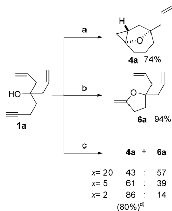
Scheme 3. Different reaction conditions for the cycloisomerization reaction of the alkynol derivative 1a . a) 25 mol % [(thf)W(CO) 5 ], THF, RT; b) 5 mol % [W(CO) 6 ], 200 mol % Et 3 N, THF, 50 °C, hν ; c) 5 mol % [W(CO) 6 ], x mol % Et 3 N, THF, 50 °C, hν . d) Isolated yield of 4a when x = 2.
