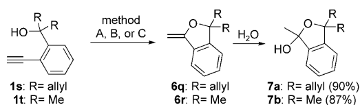
Scheme 4. Cycloisomerization reactions of the o -ethynylbenzyl alcohols 1s , t . Method A: 25 mol % preformed [(thf)W(CO) 5 ], THF, RT; method B: 10 mol % [W(CO) 6 ], 2 mol % Et 3 N, THF, 50 °C, hν ; method C: 10 mol % [W(CO) 6 ], 200 mol % Et 3 N, THF, 50 °C, hν .
