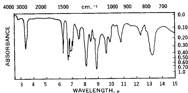
Figure 1—Infrared curve of 3-(3,4-methylenedioxybenzyl)-4-(3',4',5'-trimethoxybenzyl) tetrahydrofuran (burseran).
