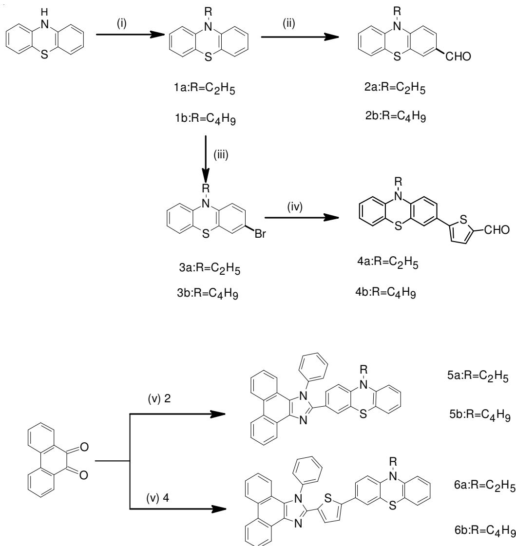
Scheme-I: Synthetic route to 5a , 5b , 6a and 6b . Reagents and conditions: (i) \text{NaOH} , DMSO, rt; (ii) DMF, \text{POCl}_3 , reflux; (iii) NBS, DMF, rt; (iv) \text{Pd}(\text{PPh}_3)_4 , 1\text{ M Na}_2\text{CO}_3 , 1,2-dioxane, reflux; (v) phenanthraquinone, ammonium acetate, glacial acetic acid, 140^\circ\text{C}
