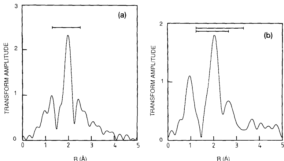
Fig. 2. Fourier transforms of k^3 -weighted EXAFS data of magnesium bromide in (a) diethyl ether, k -range 3.0–14.5 \text{\AA}^{-1} , and in (b) tetrahydrofuran, k -range 3.0–12.7 \text{\AA}^{-1} , (b). The horizontal bars indicate the width of the windows used when back-transforming the data. R is related to the true distance R' by the phase shift \alpha according to R' = R + \alpha .
