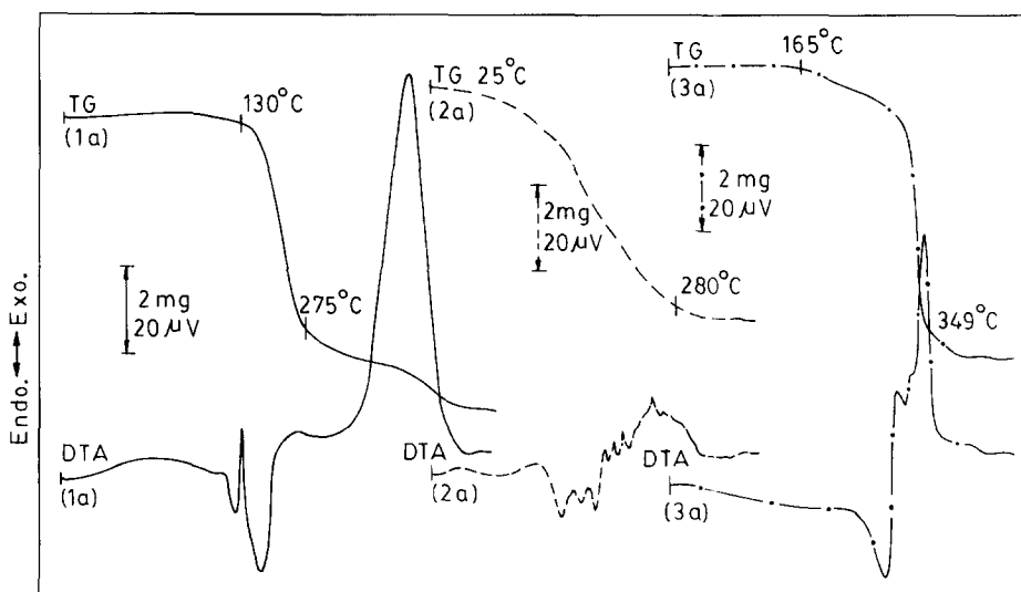
Fig. 1. Thermal curves of [\text{Pd}(\text{morph})_2\text{Cl}_2] (1a) (—), sample mass 9.4 mg; [\text{Pd}(\text{thiox})_2\text{Cl}_2] (2a) (---), sample mass 9.3 mg; and [\text{Pd}(\text{dith})_2\text{Cl}_2] (3a) (- · - · -), sample mass 10.0 mg.
