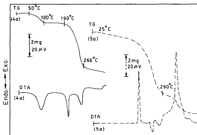
Fig. 2. Thermal curves of [Pd(Mmorph)_2Cl_2] \cdot 2H_2O (4a) (—), sample mass 6.8 mg; and [Pd(DMP)_2Cl_2] (5a) (---), sample mass 10.0 mg.
