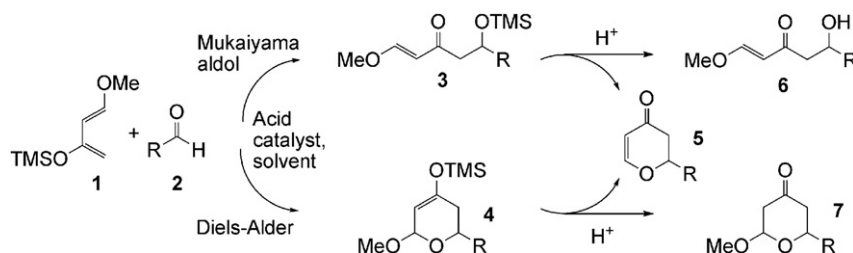
Scheme 1. The reaction of Danishefsky's diene with aldehydes. In the present study R = p -NO 2 C 6 H 4 , macrocycles 8 or 9 or dipyrromethane 10 were used as the acid catalysts, in DCM solvent.
