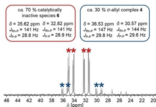
Figure 5. ^{31}\text{P} NMR spectra of the catalyzed addition of [benzoic acid] = 0.47 mol/L and [1-octyne] = 0.61 mol/L using the in situ generated precatalyst [[\text{Rh}(\text{DPEPhos})(\mu_2\text{-Cl})_2]_2] 7 = 0.023 mol/L in 1,2-dichloroethane- d_4 at 70 °C after 900 minutes; \sigma -allyl complex (4, *); unknown species which may be catalytically inactive (6, **).
