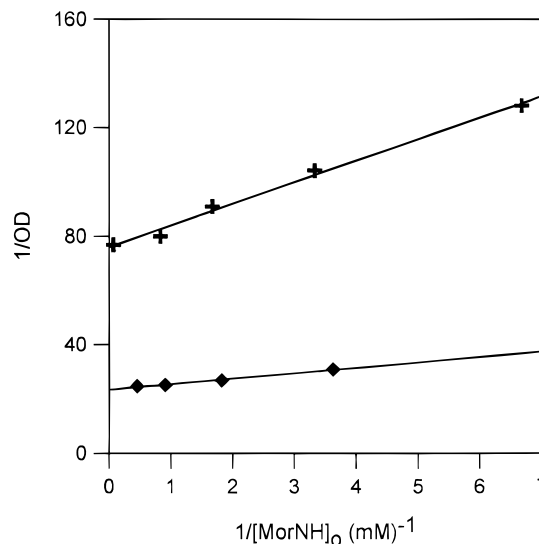
Figure 5. Double reciprocal plot of the absorbance of MorNNO with varying concentrations of MorNH in the presence of (+) 0.286 mM \cdot\text{NO} and 0.933 mM \text{O}_2 ( \blacklozenge ) 1.43 mM \cdot\text{NO} and 0.187 mM \text{O}_2 . All solutions contained 2 mM phosphate buffer at pH 7.4 \pm 0.1 .
