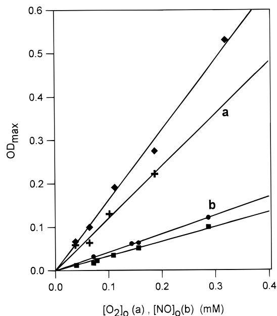
Figure 2. Measured OD at the end of the formation of SNAP and CysSO at 340 and 338 nm, respectively, in the presence of 1–4 mM thiol at pH 7.4 \pm 0.1 (1.2–1.9 mM phosphate buffer) and (a) under limiting concentration of O_2 , (♦) SNAP, (+) CysNO and (b) under limiting concentration of \cdot NO , (●) SNAP, (■) CysSNO.
