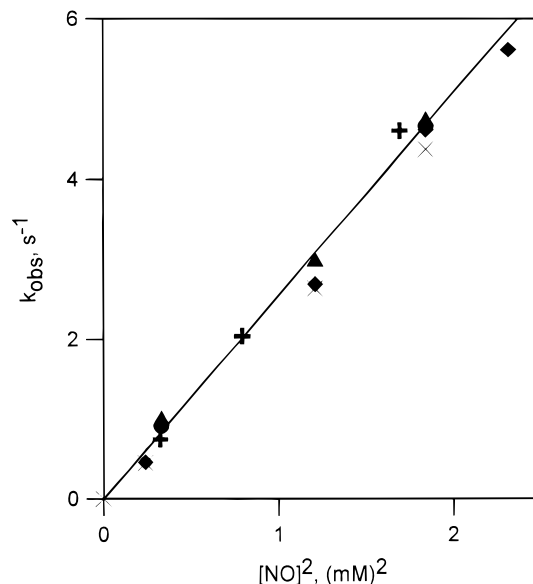
Figure 1. Observed first-order rate constant of the formation of RSNO and MorNNO as a function of [\cdot\text{NO}]^2 in the presence of 20.4–102 \mu\text{M} \text{O}_2 at pH 7.4 \pm 0.1 (1–2 mM phosphate buffer), and the following substrates: (◆) GSH; (×) CysSH; (▲) NAPenSH; (+) DTT; (●) MorNH. [\cdot\text{NO}] was taken as [\cdot\text{NO}]_0 - 2[\text{O}_2]_0 .
