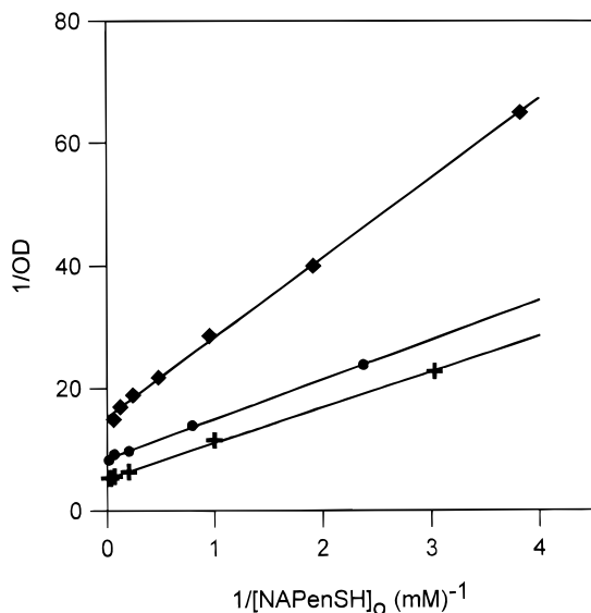
Figure 4. Double reciprocal plot of the absorbance of SNAP with varying concentrations of NAPenSH in the presence of (+) 0.86 mM \cdot\text{NO} and 0.112 mM \text{O}_2 and ( \blacklozenge ) 1.43 mM \cdot\text{NO} and 37.3 \mu\text{M} \text{O}_2 . All solutions contained 1.9 mM phosphate buffer at pH 7.4 \pm 0.1 .
