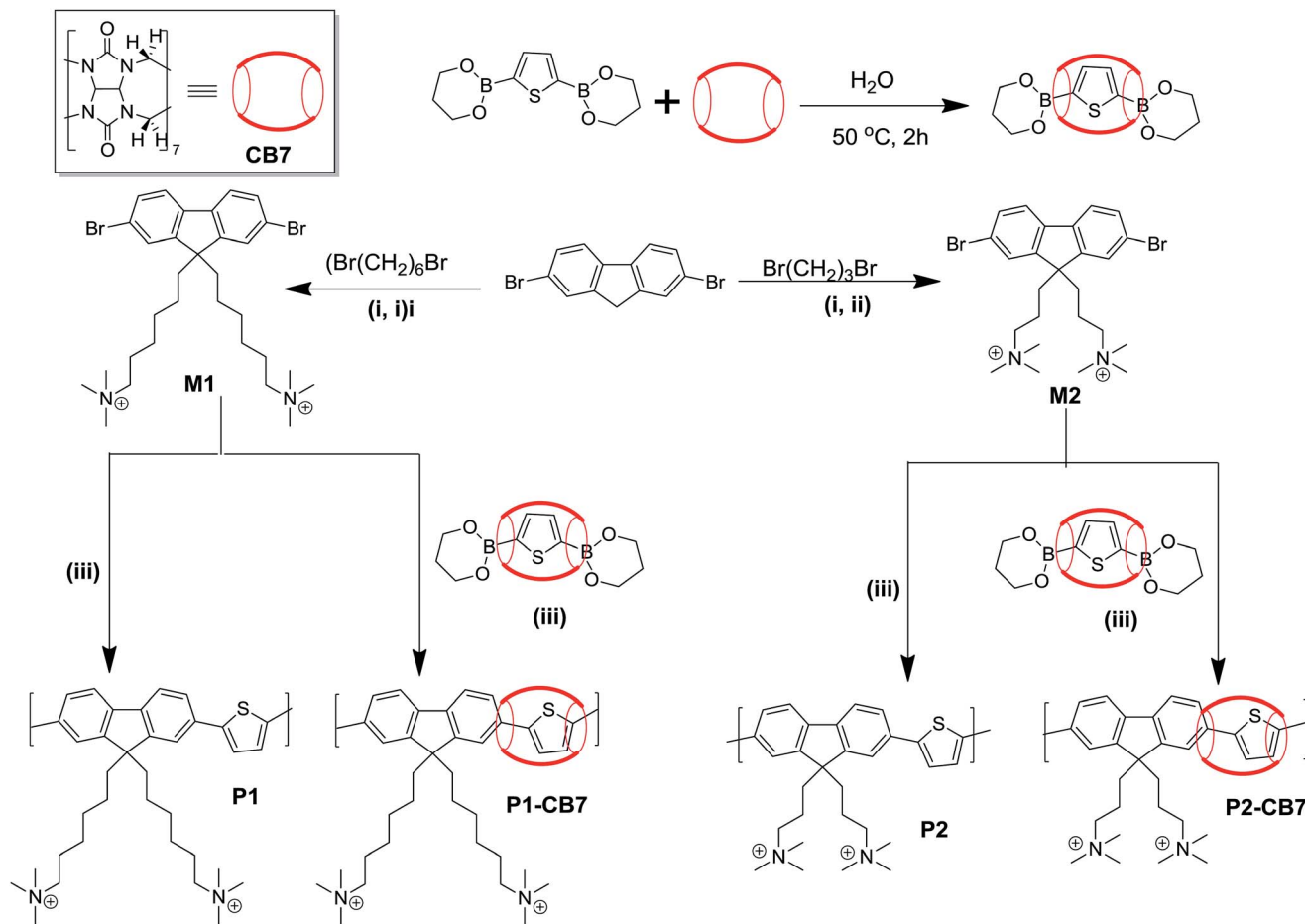
Scheme 1 Synthetic schemes for poly[9,9-bis(6( N,N,N -trimethylamino)hexyl)fluorene-co-2,5-thienylene (P1), poly[9,9-bis(3( N,N,N -trimethylamino)propyl)fluorene-co-2,5-thienylene (P2) and their CB7-based polyrotaxane counter parts P1CB7 and P2CB7. Reaction conditions: (i) TBAB, 50% wt NaOH (aq), DMSO; (ii) Me 3 N, THF, 25 °C, 24 h; (iii) Pd(OAc) 2 , K 2 CO 3 , H 2 O, 80 °C, 48 h.
