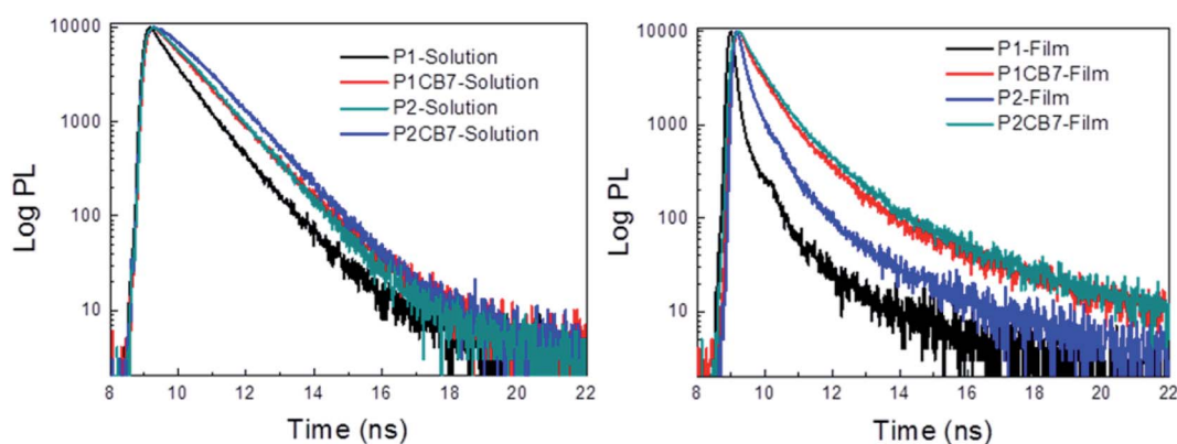
Fig. 6 Biexponentially fitted fluorescence lifetime decay curves of P1 , P2 , P1CB7 and P2CB7 in aqueous media and in solid state.
