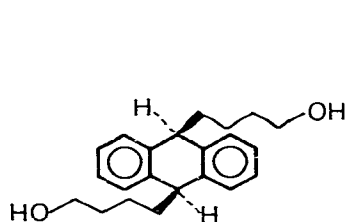
Fig. 5. 9,10-Bis(4-hydroxybutyl)-9,10-dihydroanthracene (III). ^1\text{H} NMR, \delta (TMS) ( \text{CDCl}_3 ): 7.22 (s, phenyl, 8H), 3.86 (t, benzylic, 2H), 3.58 (t, \text{CH}_2\text{OH} , 4H), 2.1 (s, OH, 2H), 1.62 ppm (m, methylene, 12H). ^{13}\text{C} NMR, \delta (TMS) ( \text{CDCl}_3 ): 139.9 (q), 128.7, 126.0, 62.7, 46.6, 42.2, 32.8, 24.7 ppm.
