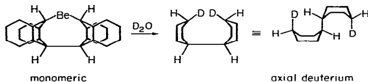
Fig. 4. Hydrolysis of a cyclic monomeric beryllium structure leads to a different H\text{-}d_2 . Some benzo rings have been omitted for clarity.
