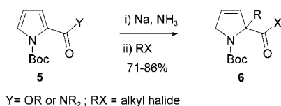
Scheme 1. General sequence for the reductive alkylation of a pyrrole.
