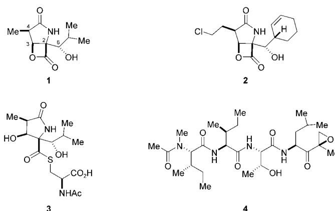
Figure 1. Examples of potent and selective proteasome inhibitors.
