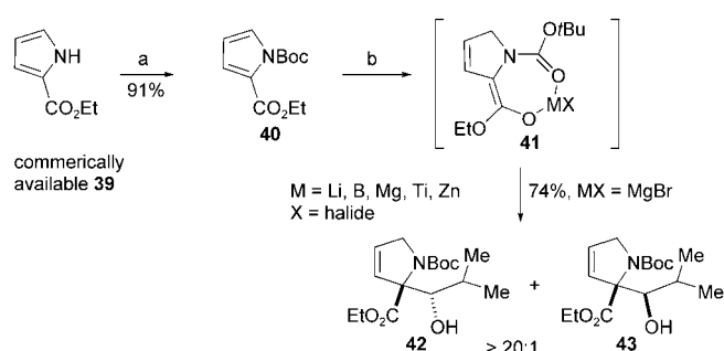
Scheme 8. Reductive aldol reaction on an electron deficient pyrrole: a) (Boc) 2 O, DMAP, Et 3 N, CH 2 Cl 2 ; b) Li, DBB, THF, −78 °C, (MeOCH 2 CH 2 ) 2 NH, MX, isobutyraldehyde.
