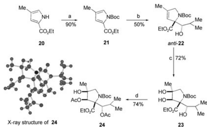
Scheme 4. Reductive aldol and oxidative manipulation reactions: a) (Boc) 2 O, Et 3 N, MeCN, DMAP, RT; b) Li, naphthalene, BMEA, THF, -78°C; iPrCHO, then NH 4 Cl aq.; c) cat. OsO 4 , NMO, acetone/H 2 O, RT; d) Ac 2 O, pyridine, cat. DMAP.
