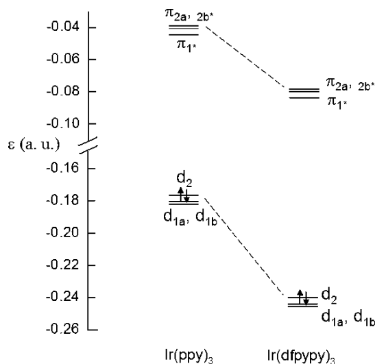
Figure 7. Schematic drawing of orbital energies of highest occupied and lowest unoccupied MOs of Ir(dfpypy) 3 from B3LYP calculations. The orbital energies of Ir(ppy) 3 were cited from ref 9 for the purpose of comparison. HOMO, HOMO - 1, and HOMO - 2 were denoted d_2 , d_{1a} , and d_{1b} . LUMO, LUMO + 1, and LUMO + 2 were denoted \pi_{1^*} , \pi_{2a^*} , and \pi_{2b^*} . (1 au = 27.212 eV)
