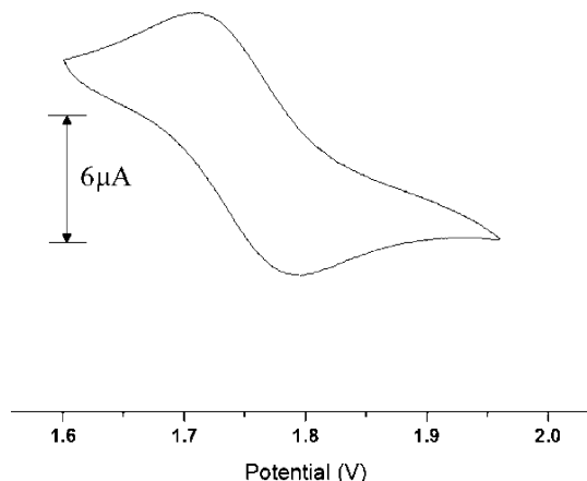
Figure 5. Cyclic voltammograms of 1 in 0.1 M n -Bu 4 NPF 6 at a scan rate of 100 mV/s.
