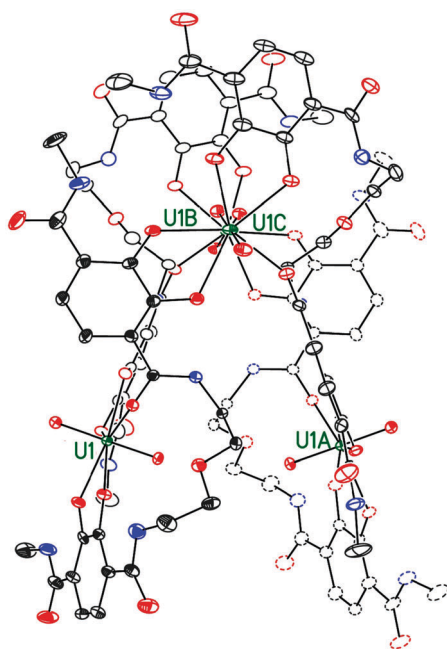
Fig. 1 Crystal structure of [\text{LUO}_2]_4^{8-} (30% probability) without hydrogen atoms. The four ligands are presented in four different ellipsoid formats. Carbon atoms are grey, nitrogen atoms blue, oxygen atoms red, and uranium atoms green.
