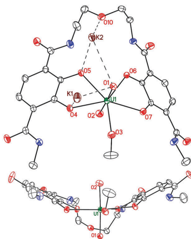
Fig. 2 Crystal structure of [\text{LUO}_2(\text{OMe})]^{3-} (30% probability) without hydrogen atoms. Up: structure of [\text{K}_2\text{LUO}_2(\text{OMe})]^- ; down: side view of [\text{LUO}_2(\text{OMe})]^{3-} .
