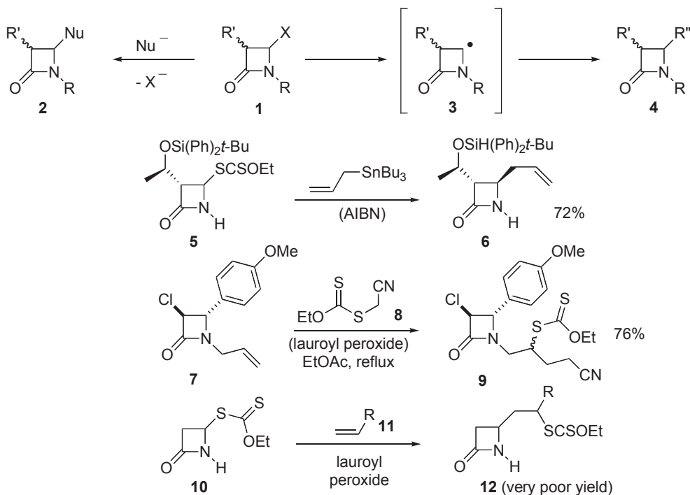
Scheme 1. Modification of \beta -lactams
