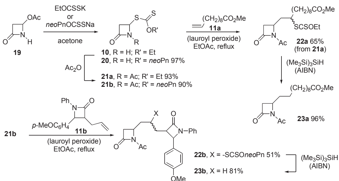
Scheme 3. Radical additions of S -azetidiny xanthates
