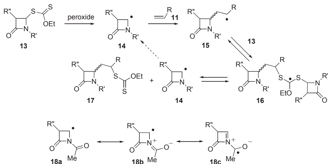
Scheme 2. Simplified mechanistic rationale
