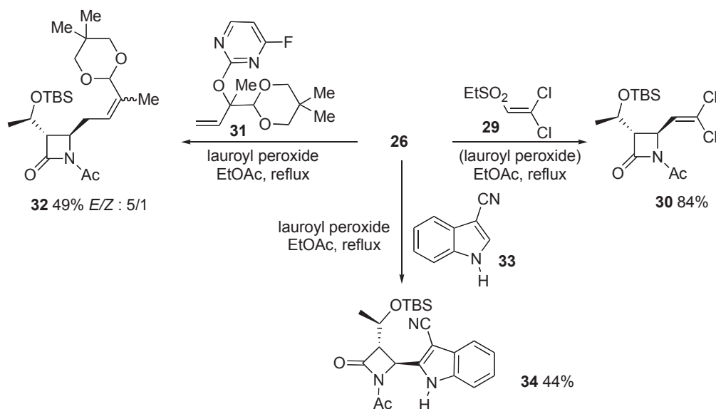
Scheme 5. Radical vinylation, allylation and heteroarylation of functionalised S -azetidinyI xanthates
