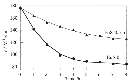
Figure 2. Time dependence absorption values indicating dispersibility of EuS-0 (20 nm) and EuS-0.5-p (21 nm).
