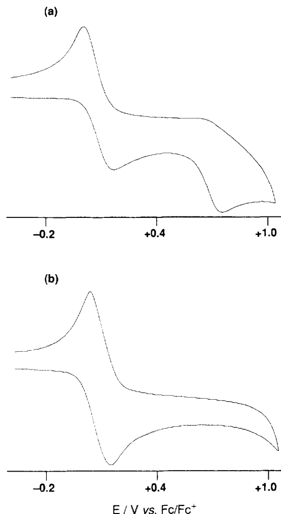
Fig. 5. Cyclic voltammograms of (a) 1 and (b) 7 , recorded in CH_2Cl_2 at a Pt-bead working electrode with a scan rate of 0.2 \text{ V s}^{-1} .
