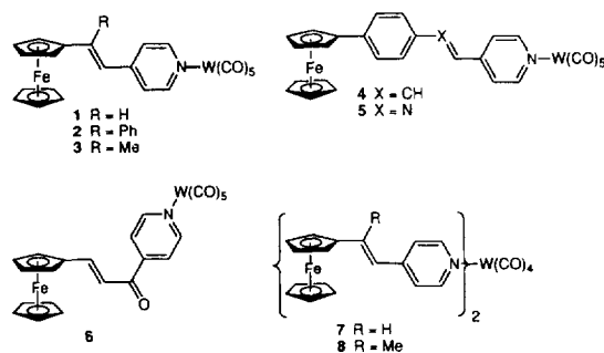
Fig. 1. Structural formulae of the new complexes.
