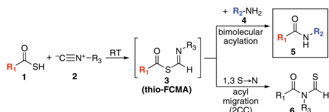
Figure 2. Proposed base-free amide \beta -asparagine linkage through interception of a thio-FCMA (formimide carboxylate mixed anhydride) intermediate.
