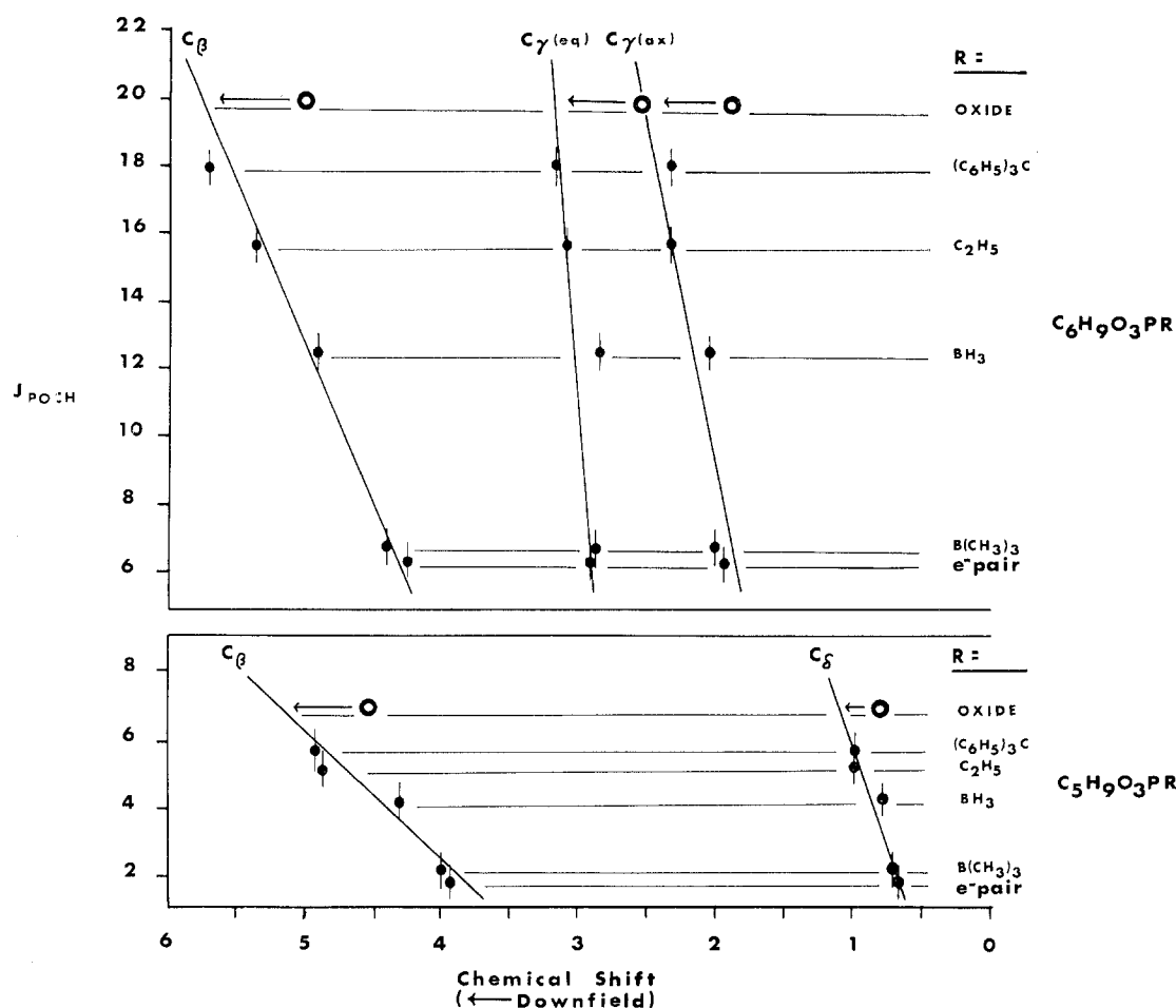
Figure 4.—Spin coupling (c.p.s.) of P to H on C_\beta carbons ( J_{POCH} ) vs. chemical shift (—p.p.m. with respect to tetramethylsilane) of protons in C_5H_9O_3P (I) and C_6H_9O_3P (II) and their B(CH_3)_3 , BH_3 , C_2H_5 , (C_6H_5)_3C , and oxide derivatives.
