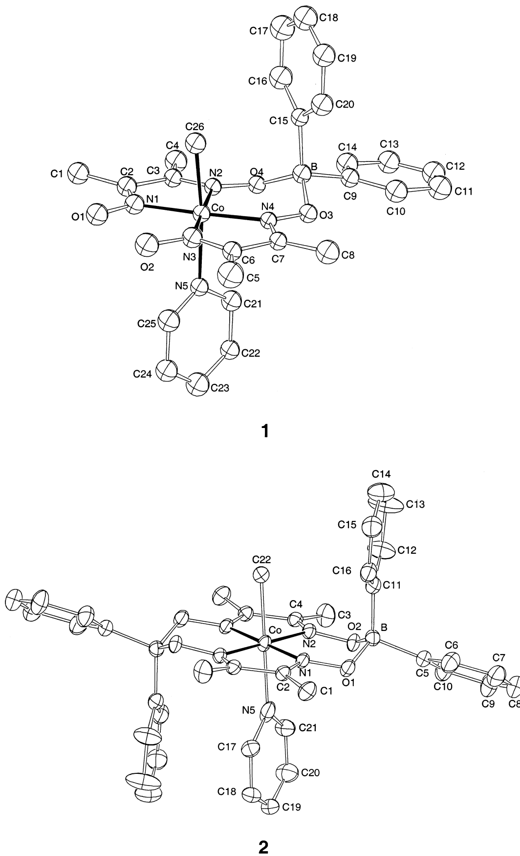
Fig. 1. The ORTEP drawing and the atom numbering scheme of the complexes MeCo(DH)(DBPh 2 )Py (1) and MeCo(DBPh 2 ) 2 Py (2) (thermal ellipsoids at 30% probability).
