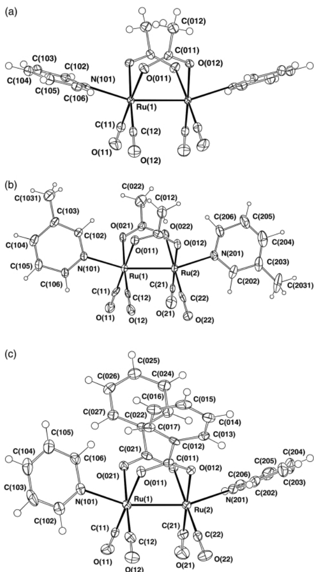
Fig. 1 Projections of representative arrays of the [\text{Ru}(\text{RCO}_2)(\text{CO})_2\text{L}]_2 systems: (a) \text{R} = \text{Me} , \text{L} = \text{py} , showing the 2 \times \text{flat} ( \text{N-base} ) _2 disposition; (b) \text{R} = \text{Me} , \text{L} = \text{Mepy} , (molecule 1; the other molecule is similar) showing the 2 \times \text{upright} ( \text{N-base} ) _2 disposition of the nitrogen bases; (c) \text{R} = \text{Ph} , \text{L} = \text{py} , showing the 1 \times \text{flat} , 1 \times \text{upright} ( \text{N-base} ) _2 disposition.
