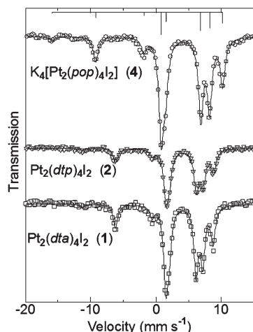
Figure 2. ^{129}\text{I} Mössbauer spectra of the MMX chain precursors 1 , 2 , and 4 .
