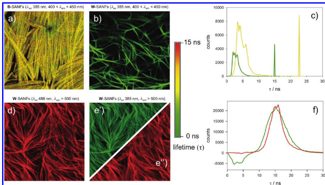
Figure 6. (a, b, d, e) Confocal FLIM images ( 30 \times 30 \mu\text{m} ) with color codes green, yellow, and red representing average decay times from shorter to longer: (a) B-gel, (b, d, e) W-gel, (a, b) \lambda_{ex} = 385 nm, 400 \text{ nm} < \lambda_{em} < 450 nm, (d) \lambda_{ex} = 488 nm, \lambda_{em} > 500 nm, (e', e'') \lambda_{ex} = 385 nm, \lambda_{em} > 500 nm, (e') rise, (e'') decay. (c) Histograms of decay time \tau distributions obtained by triexponential fitting of decays of (yellow) image a and (green) image b. (f) \tau distributions obtained by (red) exponential fitting of decays of image d and (green) biexponential fitting of transient emission of image e. Decay = positive, and rise = negative.
