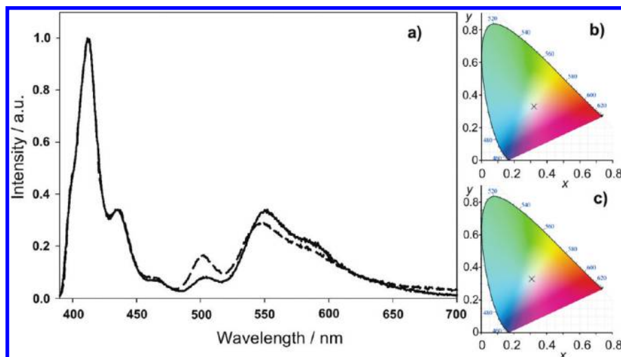
Figure 3. (a) Corrected fluorescence spectra ( \lambda_{\text{ex}} = 365 nm) of (full line) a W -gel/DMSO and (dashed line) a W -gel/MeOH. (b) CIE 1931 chromaticity coordinates of W -gel/DMSO: x = 0.319 , y = 0.332 . (c) CIE 1931 chromaticity coordinates of W -gel/MeOH: x = 0.306 , y = 0.331 .
