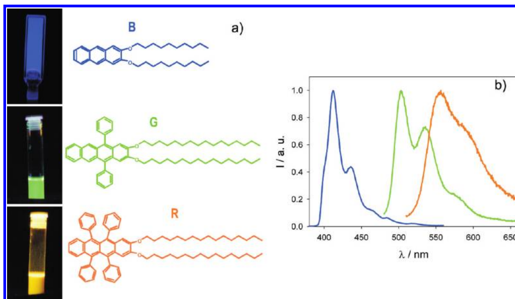
Figure 1. (a) Pictures of a 2 mM B gel in DMSO, 10 \mu M G solution in THF, and 10 \mu M R solution in THF under UV light ( \lambda_{\text{ex}} = 365 nm) and the molecular structures. (b) Corrected fluorescence spectra of B , G , and R ( \lambda_{\text{ex}} = 365 nm).
