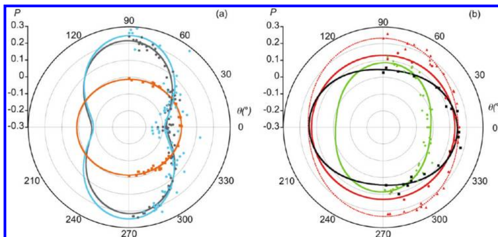
Figure 8. Polar plots of average P for individually picked SANF segments (2–5 \mu\text{m} long) as a function of the angle \theta of the fiber axis with respect to the laser polarization (east/west): (a) \lambda_{\text{ex}} = 385 nm, (gray circles) B -SANFs, \lambda_{\text{em}} > 405 nm, (blue circles) W -SANFs, 400 \text{ nm} < \lambda_{\text{em}} < 450 nm, (orange squares) \lambda_{\text{em}} > 500 nm; (b) \lambda_{\text{ex}} = 488 nm, \lambda_{\text{em}} > 500 nm, (black squares) W -SANFs, (green tilted squares) B + G (1.2%), (full red circles) B + R (1.2%), (red triangles) B + R (0.05%). Full lines are guides to the eye only and are obtained by fitting P with a simple sinusoidal function.
