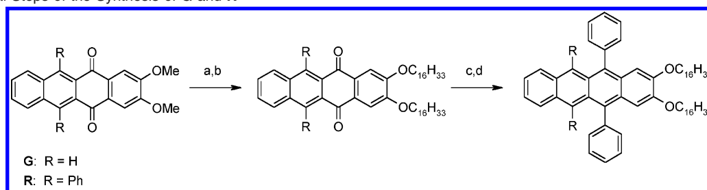
Scheme 1. Final Steps of the Synthesis of G and R a
