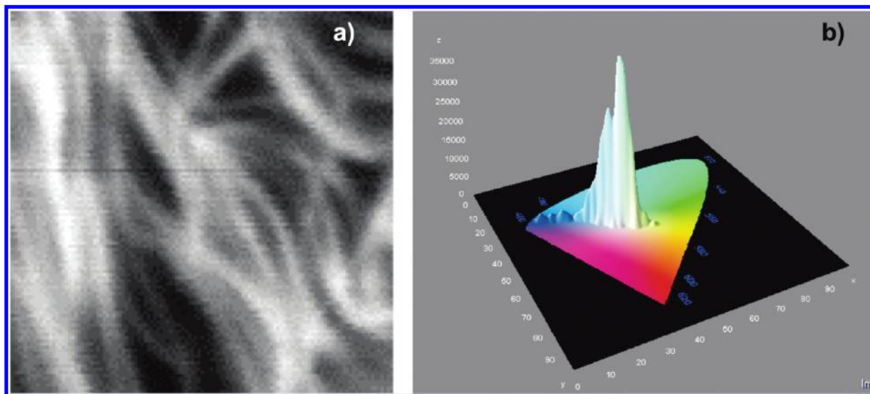
Figure 5. (a) Fluorescence intensity confocal microscopy image ( 20 \times 20 \mu\text{m} ) of a W -gel (DMSO) at 22^\circ\text{C} ( \lambda_{\text{ex}} = 385 \text{ nm} , \lambda_{\text{em}} > 405 \text{ nm} ). (b) Distribution of the CIE 1931 chromaticity coordinates of 500 fluorescence spectra, similar to Figure 4a, acquired while scanning the nanofibers in an area of 20 \times 20 \mu\text{m} . The z -scale represents the number of photons yielding the given coordinates.
