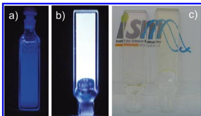
Figure 2. (a, b) Pictures of cuvettes with 2.0 mM B with 0.012 equiv of G and R under UV light, \lambda_{\text{ex}} = 365 nm: (a) THF solution, (b) DMSO organogel ( W-gel ). (c) Pictures of quartz cuvettes containing pristine B organogel ( B-gel ) and W-gel under daylight (the logo of our institute can be seen in the background through the translucent gels).
