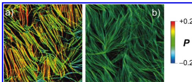
Figure 7. Fluorescence polarization confocal images ( 30 \times 30 \mu\text{m} ) under horizontally polarized excitation (east/west, \lambda_{ex} = 385 nm) of a W-gel: (a) 400 \text{ nm} < \lambda_{em} < 450 nm, (b) \lambda_{em} > 500 nm. Color codes correspond to the polarization P : from negative to positive, blue, green, and red.
