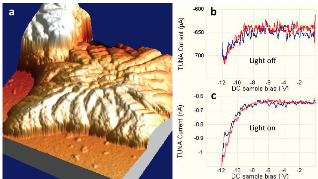
Figure 8. AFM image ( 5\ \mu\text{m} \times 5\ \mu\text{m} ) of a \text{ZnTPPS}^{4-} and \text{SnT}(\text{N-EtOH-4-Py})\text{P}^{4+} clover (a) and TUNA current–voltage curve for conduction to the AFM Ti/Pt tip at a point on the clover surface through the clover from a p-doped conductive Si substrate with 20 ohm cm resistivity in the dark (b) and when illuminated with the cold incandescent lamp of the AFM instrument (c).
