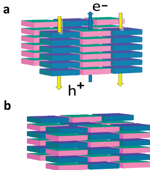
Figure 10. Idealized packing for donor–acceptor solids: (a) segregated stacking and (b) interleaved stacking. 36 As drawn, the blocks in panel a would represent H-aggregates, so the stacks must actually be tilted to represent the slipped stacks of J-aggregates. Slipped stacks would still produce the columns of charges at the corners as discussed in the text.
