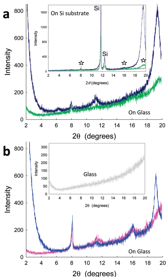
Figure 6. (a) XRD data for Sn/Zn clovers [ \text{SnTPPS}^{4-} and \text{ZnT}(\text{N-EtOH-4-Py})\text{P}^{4+} ] (green) and for the Zn/Sn clovers (dark blue) on glass slides. Inset: Sn/Zn (green) and Zn/Sn (dark blue) clovers on the Si wafer and the Si substrate (gray); the stars indicate reflections from the clovers. (b) XRD data for the Zn/Zn clovers (blue) and Sn/Sn clovers (pink) on glass (inset). All samples are dried as follows: Sn/Zn, Sn/Sn, and Zn/Zn by mild heating and Zn/Sn at room temperature.
