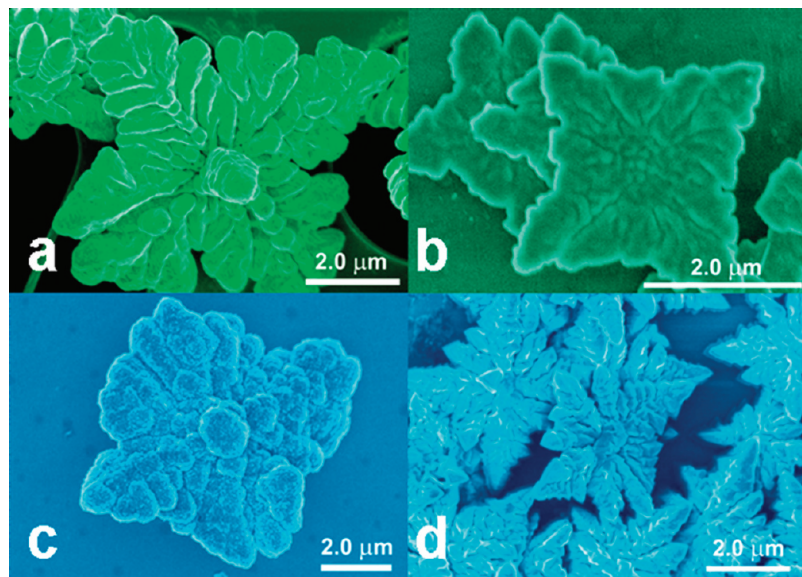
Figure 5. Cloverlike structures obtained from (a) \text{SnTPPS}^{4-} and \text{ZnT}(\text{N-EtOH-4-Py})\text{P}^{4+} , (b) \text{ZnTPPS}^{4-} and \text{SnT}(\text{N-EtOH-4-Py})\text{P}^{4+} , (c) \text{SnTPPS}^{4-} and \text{SnT}(\text{N-EtOH-4-Py})\text{P}^{4+} , and (d) \text{ZnTPPS}^{4-} and \text{ZnT}(\text{N-EtOH-4-Py})\text{P}^{4+} .
