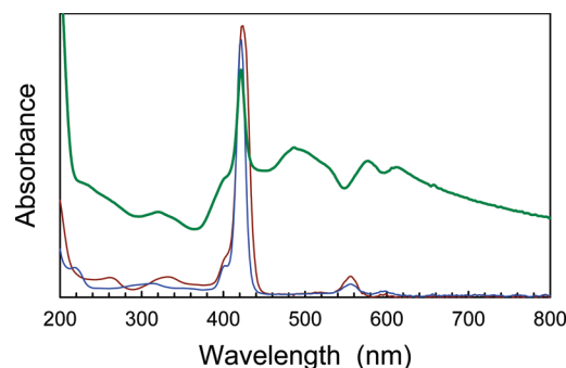
Figure 7. UV-visible absorption spectra of a suspension of the Zn/Sn clovers (green) and the constituent porphyrins \text{ZnTPPS}^{4-} (blue) and \text{SnT}(\text{N-EtOH-4-Py})\text{P}^{4+} (red). The J-aggregate band seen near 500 nm for the Zn/Sn clovers is indicative of exciton delocalization over multiple porphyrins.
