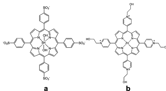
Figure 1. Structures of (a) tin(IV) tetrakis(4-sulfonatophenyl)porphyrin ( \text{SnTPPS}^{4-} ) and (b) zinc(II) tetrakis( N -ethanol-4-pyridinium)porphyrin [ \text{ZnT(N-EtOH-4-Py)P}^{4+} ].
