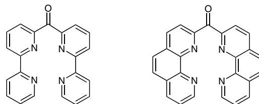
bis(2,2'-bipyrid-6'-yl) ketone ( L1 ) bis(1,10-phenanthrolin-2-yl) ketone ( L2 )
