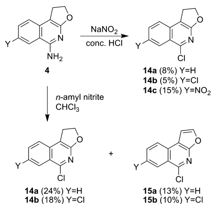
Chart 5. Deaminochlorination of 4
