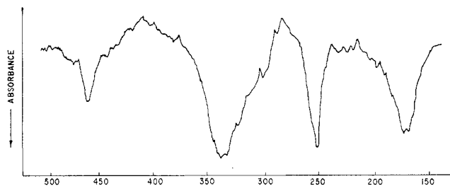
Figure 1.—Far-ir spectrum for trans -[( \text{C}_2\text{H}_5 ) _4\text{N} ][ \text{RhCl}_4(\text{CH}_3\text{CN})_2 ]. See Table III.
