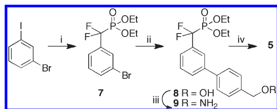
Scheme 1. Synthesis of Inhibitor Platform 5 a
