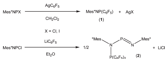
Scheme 2. Reaction of Mes^*-N=P-X with MC_6F_5 ( M = Ag, Li )
