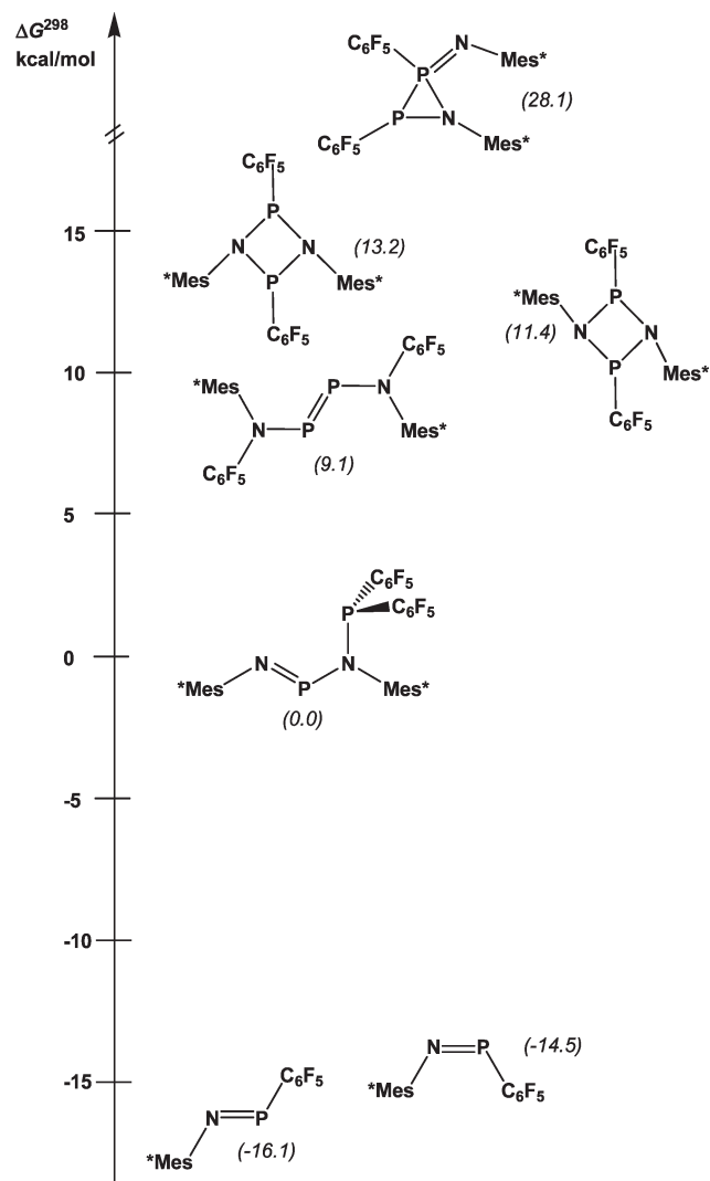
Figure 2. Relative Gibbs energies for the isomers of [\text{Mes}^*\text{NP}(\text{C}_6\text{F}_5)]_y ( y = 1, 2 ). The exact values are given in parentheses.
