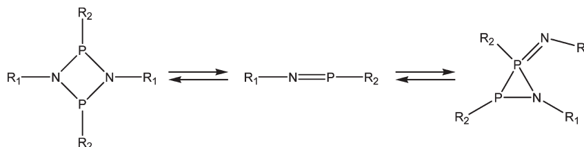
Scheme 1. Different Channels for the Dimerization of R_1-N=P-R_2
