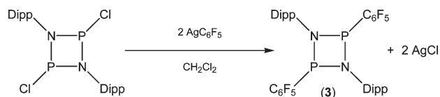
Scheme 3. Reaction of [Cl-P(\mu-N-Dipp)]_2 with AgC_6F_5
