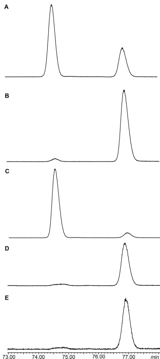
Figure 5. Total ion chromatogram of the gas chromatographic enantiomer separation of 14 on a chiral \beta -TBDMS-hydrodex phase. Temperature program: isothermal for 60 min at 110 °C, then with 2 °C/min to 160 °C, followed by a sharp ramp of 25 °C/min to 220 °C. (A) racemic mixture; (B) S - 14 ; (C) R - 14 ; (D) natural extract of a gland extract of H. cinnamomeoventris ; (E) coinjection of the natural extract and S - 14 . Peak identities were confirmed by GC/MS.
