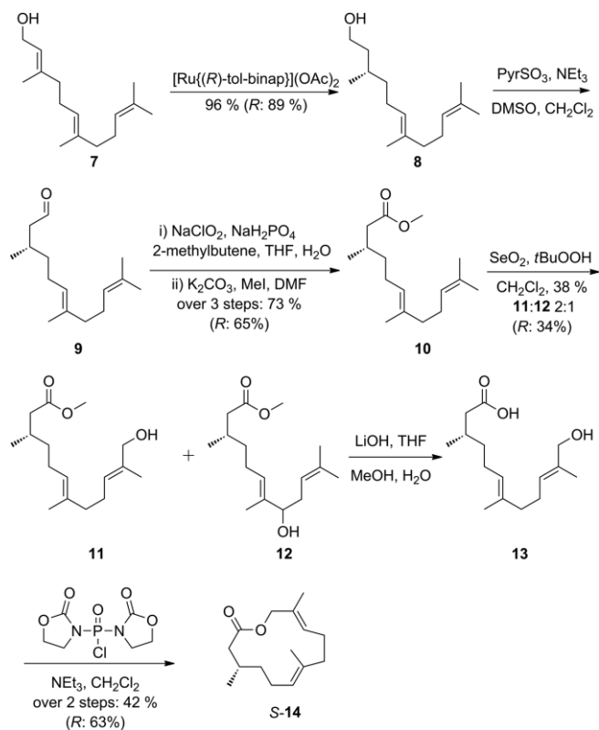
Scheme 1. Synthesis of frogolide (S-14). The synthesis was also performed with [\text{Ru}((S)\text{-tol-binap})](\text{OAc})_2 as catalyst, giving access to R-14.
