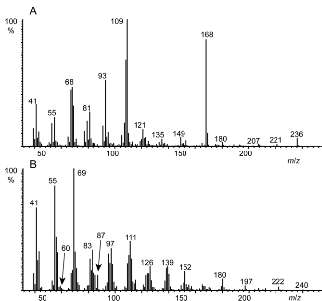
Figure 4. Mass spectra of (A) natural compound A , and (B) hydrogenated natural compound A . The shift of the M^+ -ion by 4 amu indicates the presence of two C–C double bonds in A .
