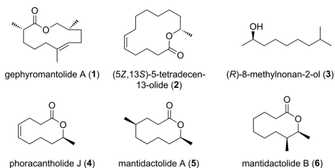
Figure 1. Compounds produced in scent glands of anuran amphibians. For compounds 3 and 4 , a species- and sex-specific, biological function has been experimentally tested.
