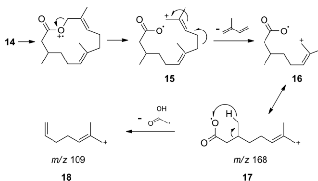
Scheme 2. Proposed fragmentation of frogolide ( 14 ) leading to the characteristic ions m/z 168 ( 17 ) and m/z 109 ( 18 ) of the mass spectrum (Figure 4A).
