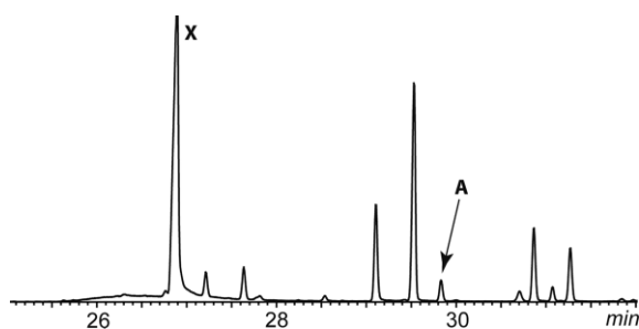
Figure 3. Total ion chromatogram of a gular gland extract of H. viridiflavus . The title compound A is indicated. X indicates a contaminant. All other peaks are oxidized sesquiterpenes of unknown structure.
